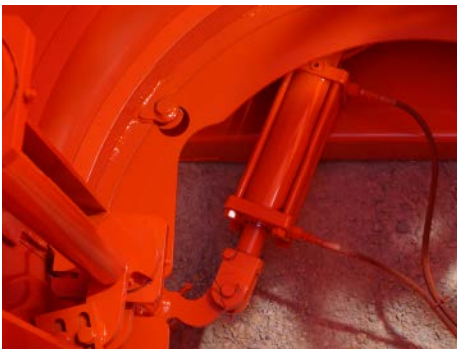
Hydraulic Core Collapsing (inside core view) 24" - 72" Diameter Cores with Quick Strip Sub-Base
