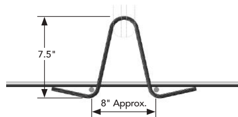
3/8" x 25" Lift Cable — Part #3825 Place cable under wire mats or rebar.
