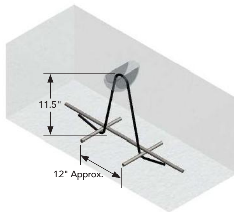
3/8" x 36" Lift Cable — Part #3836 Place cable under wire mats or rebar.
