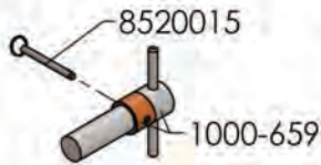
LANE EZ-LIFT LIFT PIN
