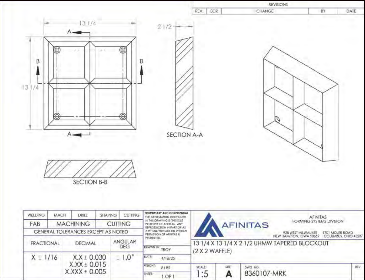
13 1/4 X 13 1/4 X 2 1/2 UHMW TAPERED BLOCKOUT (2 X 2 WAFFLE)
