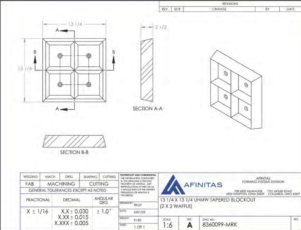
13 1/4 X 13 1/4 UHMW TAPERED BLOCKOUT (2 X 2 WAFFLE)
