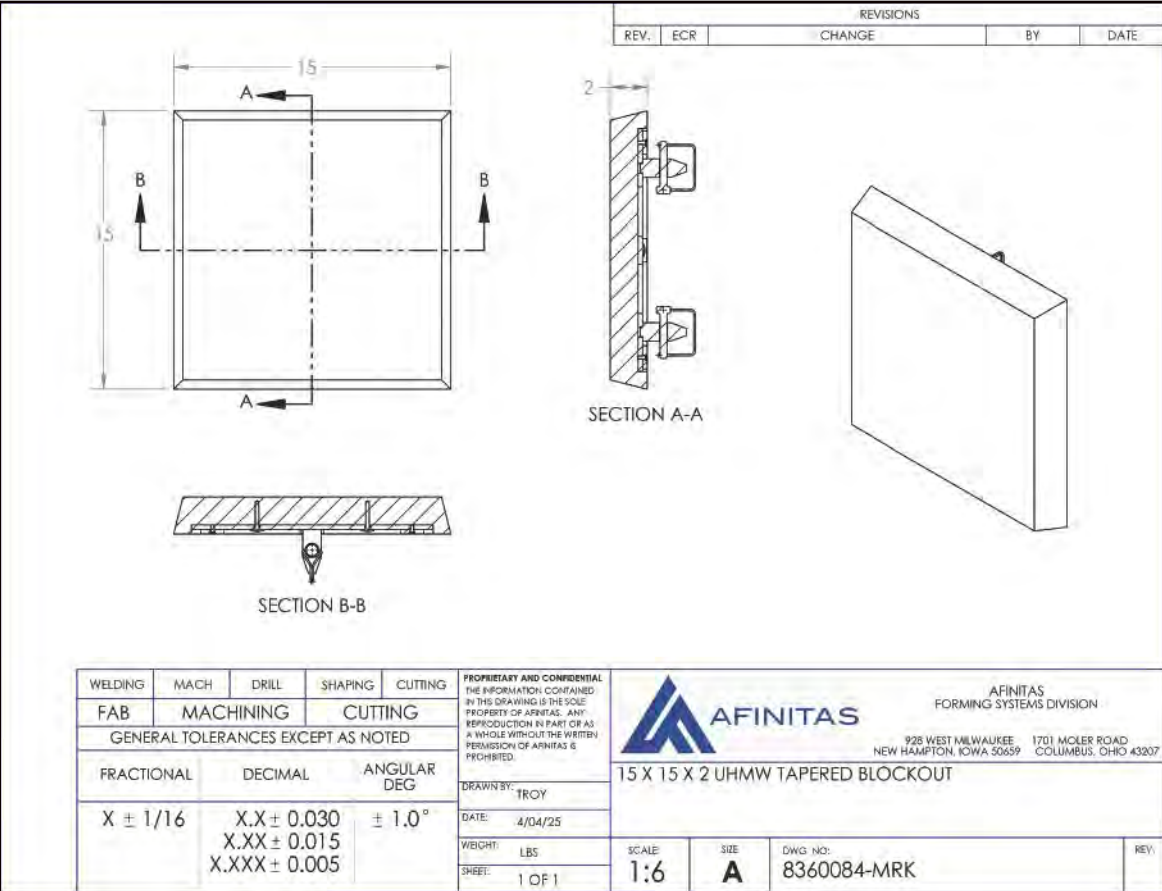
15 X 15 X 2 UHMW TAPERED BLOCKOUT
