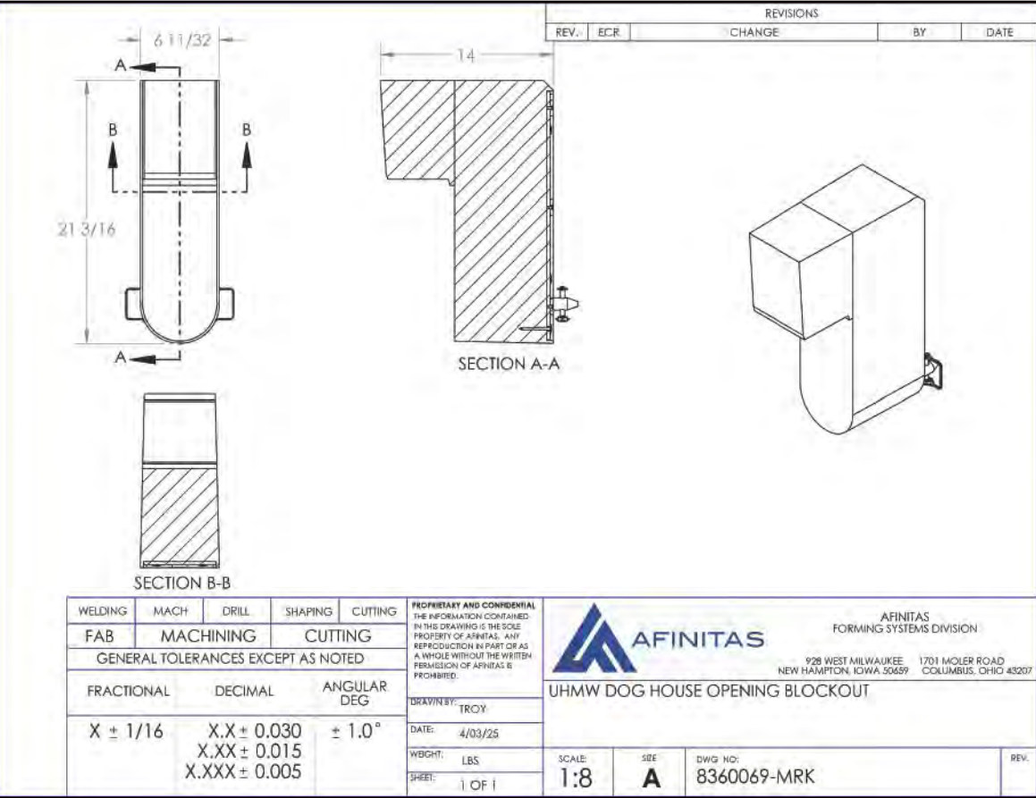
UHMW DOG HOUSE OPENING BLOCKOUT
