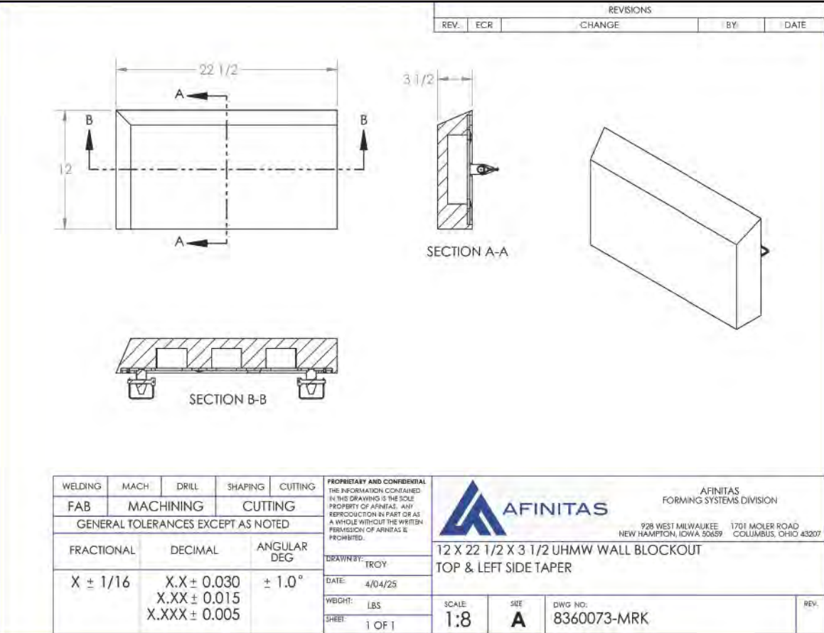
12 X 22 1/2 X 3 1/2 UHMW WALL BLOCKOUT TOP & LEFT SIDE TAPER
