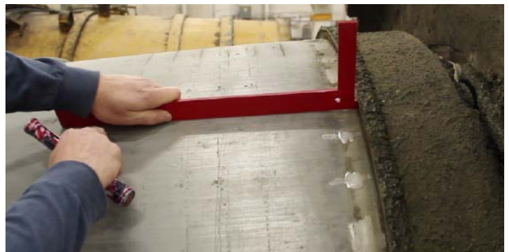
Core bottom wear and seal band inspection
